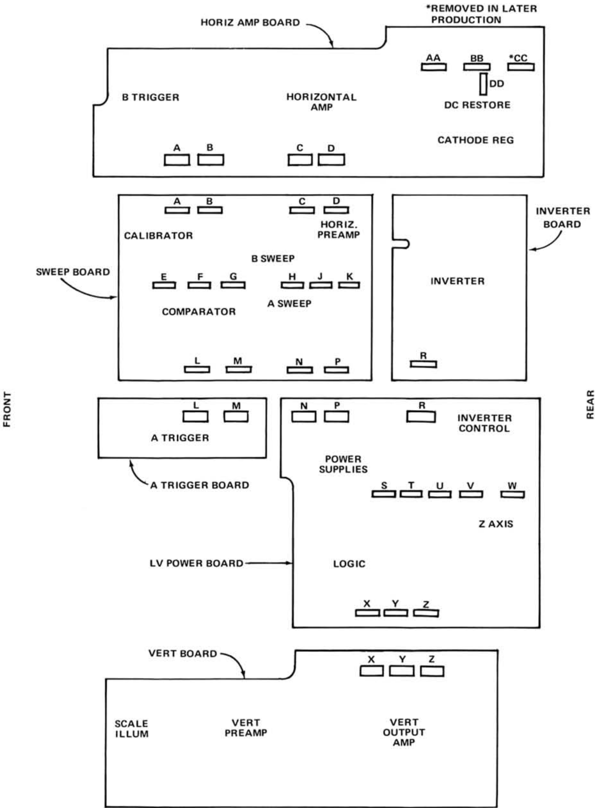
Fig. 4-3. Interboard comb connection locations.
