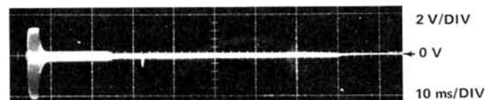
Fig. 4-2. Power Supply waveforms. Test oscilloscope internally triggered unless otherwise noted. Fig. 4-2 continued on following pages.
