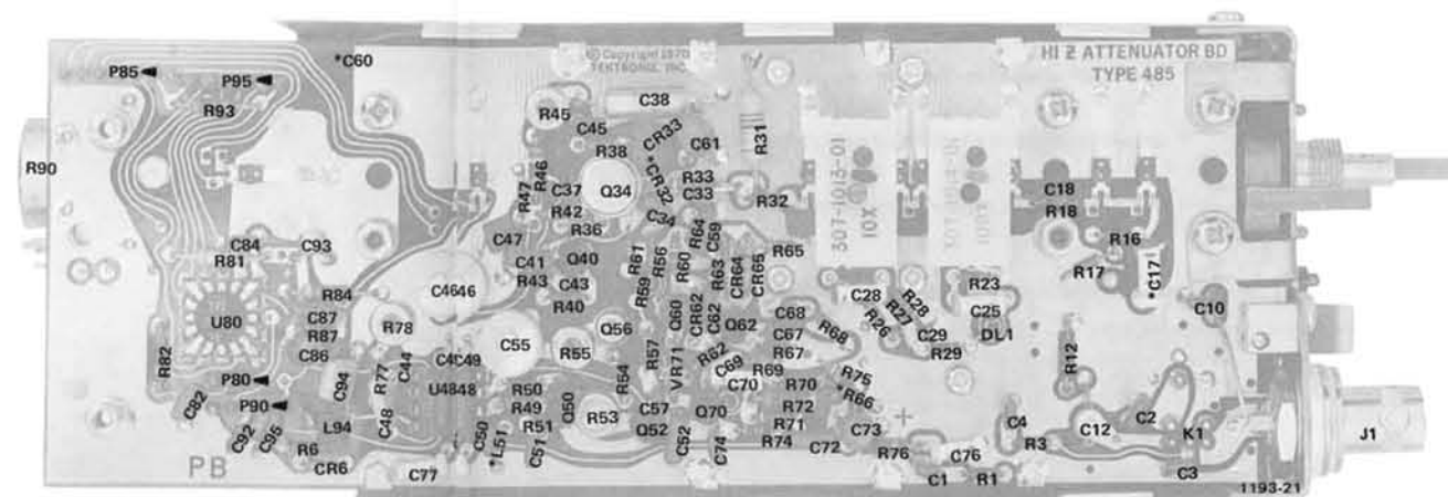
Fig. 8-2B. A. A3 Hi Z Attenuator board (485 &amp; 485-1 only) SN B010100-B155789.
