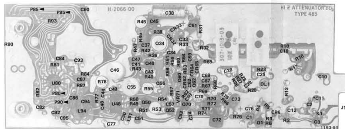
Fig. 8-2A. A3 Hi Z Attenuator board (485 &amp; 485-1 only) SN B155790-up.
