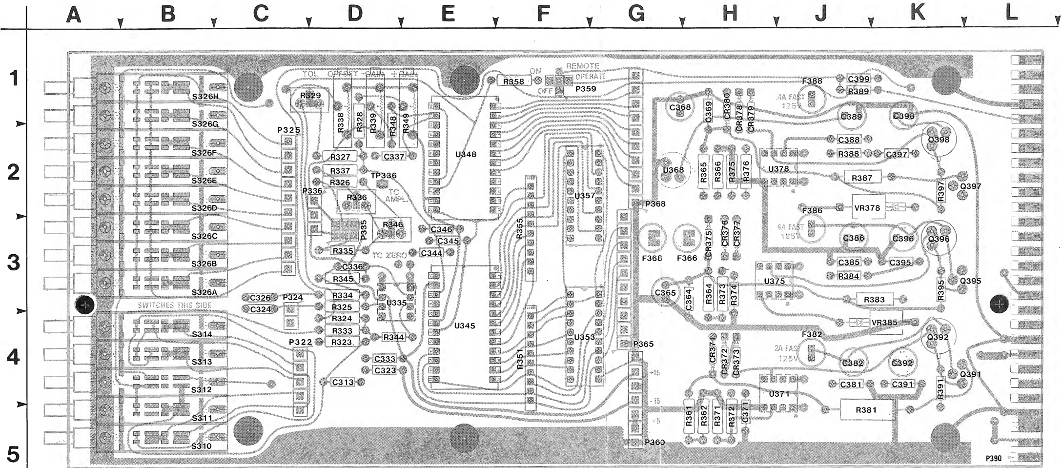
FIGURE 8-5. A3 DAC BOARD COMPONENT LOCATIONS.
