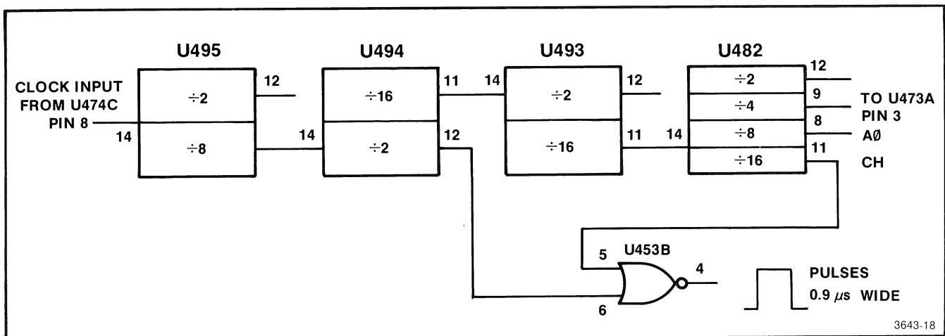
Fig. 3-3. Timebase breakdown.
