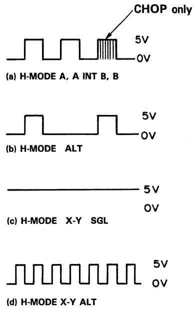
Fig. 25 Waveform
