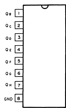
HD74HC595P
