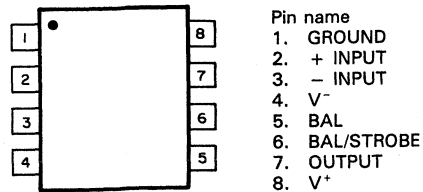
NJM311M
