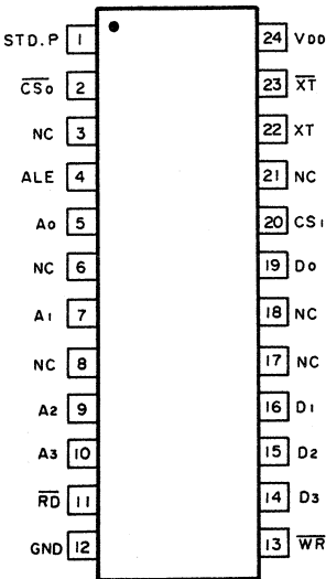
MSM6242BGS-VK
