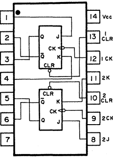
HD74LS107AFP HD74HC107FP
