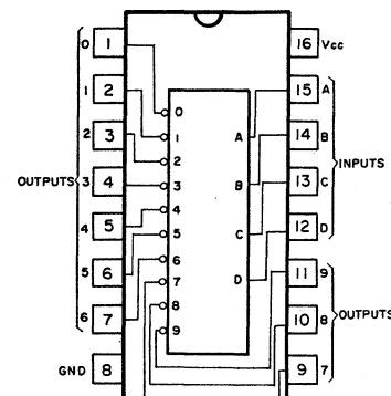
HD74LS42P
