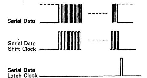
Fig. 2 Serial transmit timing chart
