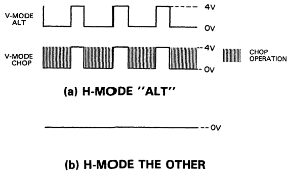
Fig. 37 U7, Pin9 Signal
