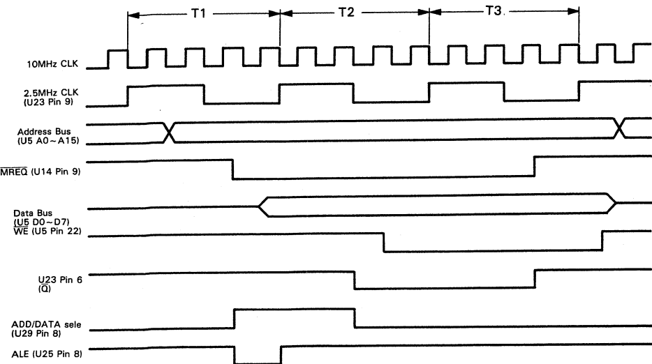
Address/Data Select Timing Chart (X77-1490-00)
