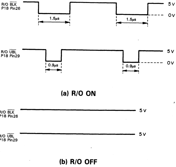
Fig. 39 P18 Pin26, 29, R/O BLK, R/O UBL Signal
