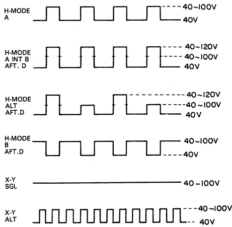
Fig. 31 Q4, Collector Signal A SWEEP TIME = B SWEEP TIME DELAY TIME MIN
