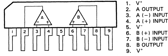
NJM072S
