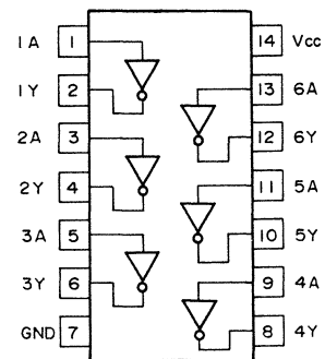
HD74LS04FP
