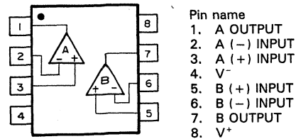
NJM072M
