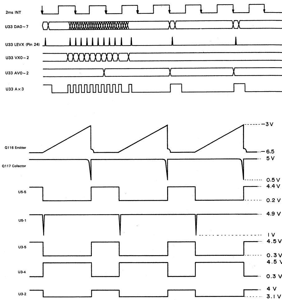
Endless VR Select and Control Timing Chart
