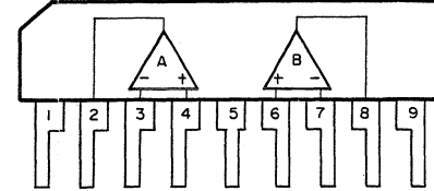
NJM4556S
