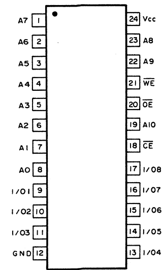
LC3517BML-15
