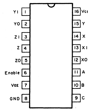
MC74HC4053N
