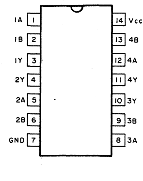
HD74HC7266FP
