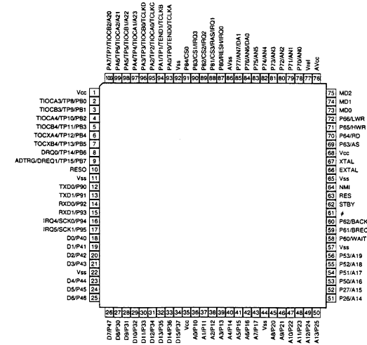
HD6433040SA00F
