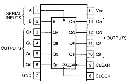
HD74LS164FP
