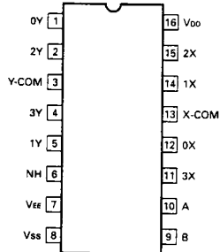
TC4052BF
