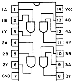
HD74LS08FP TC74HC08AF
