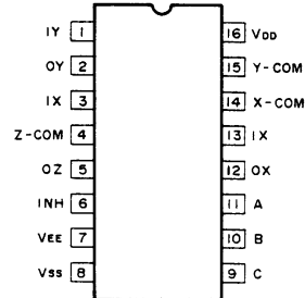
TC4053BF
