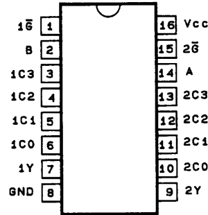
HD74LS153FP
