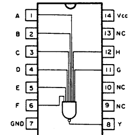
TC74HC30AF
