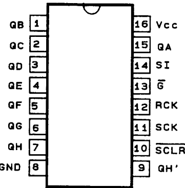
HD74HC595FP
