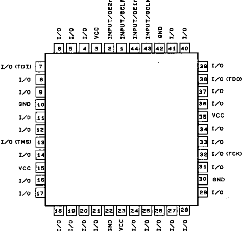
7032LC44-NAO
