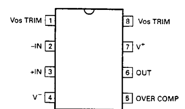
LT1097S8
