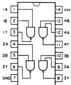
TC74HC00AF SN74ALS00ANS
