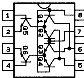
HFA3101B
