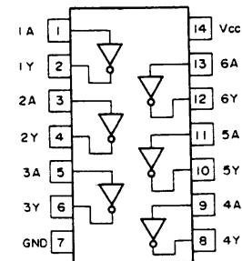
HD74LS04FP
