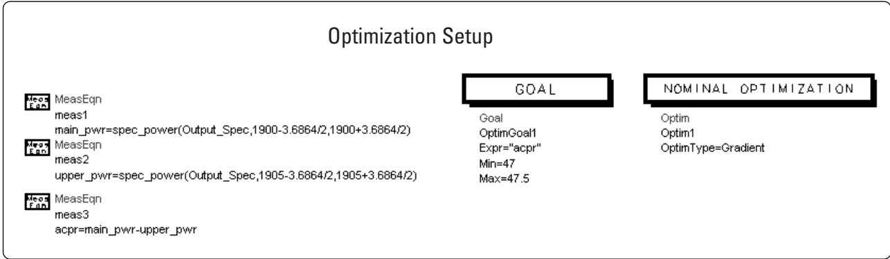
Figure 12. Setting up the simulation for optimization. In the example system, optimization setup consists of setting the minimum ACPR value to 47 dB (the desired result) and the maximum to 47.5 dB. The resulting calculation provides the minimum TOI points needed to meet the required specification.
