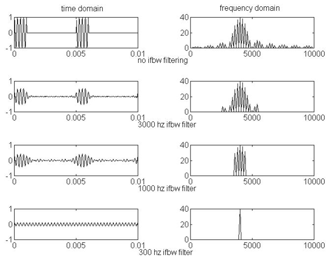
Figure 2. Effect of IF filtering on high PRF measurements
