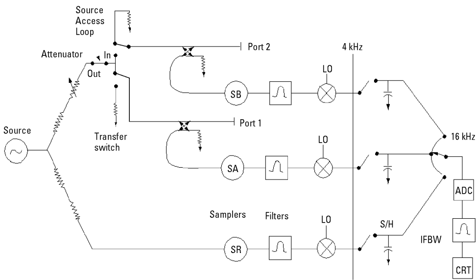
Figure 1. Network analyzer block diagram
