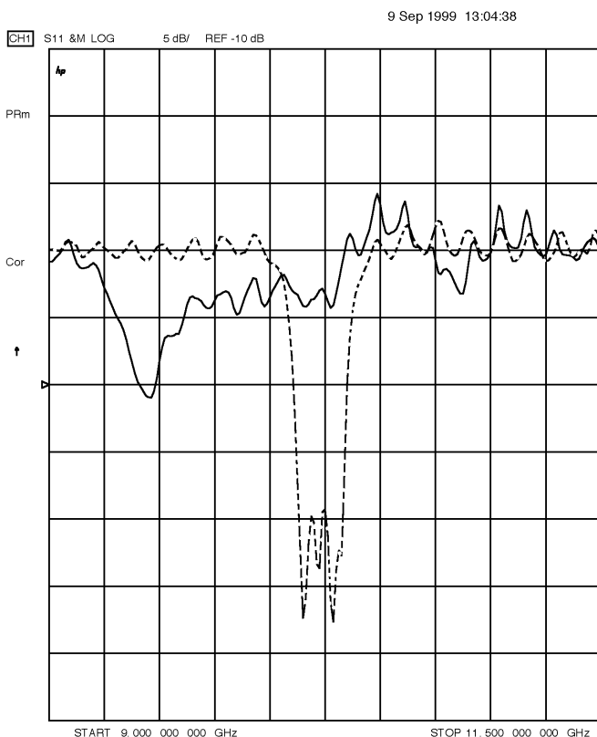
Figure 8. Valid reflection measurement in point-on-pulse mode
