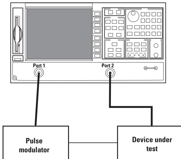
Figure 3. Simple transmission set up
