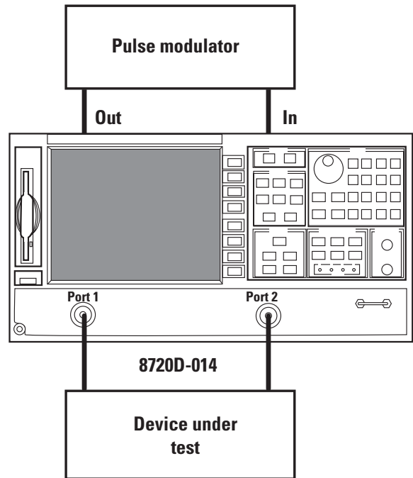
Figure 10. Pulse modulator in rear access loop (Option 014)
