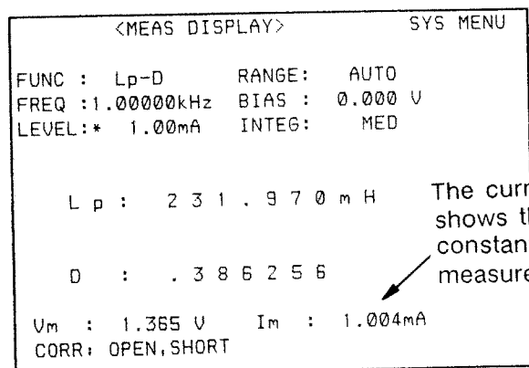
Figure 2. Constant Current L - D Measurement Example
