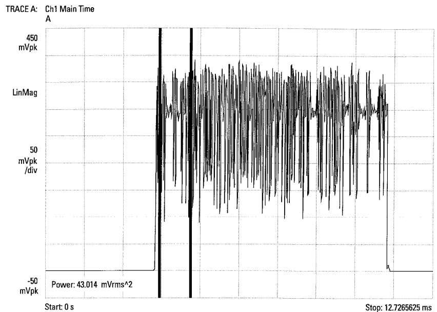
Figure 4. Use time-domain band power markers to calculate the power over a selected portion of the time-record.
