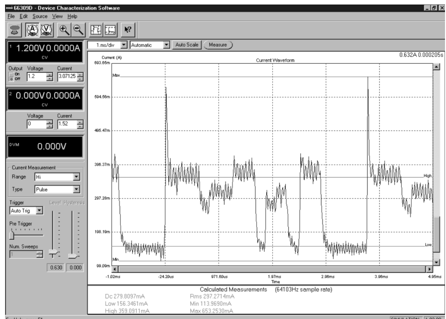
Figure 1 Example Bluetooth Headset Device Active Call Current Drain Waveform
