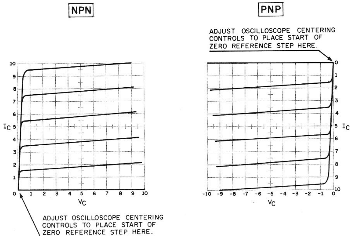
Figure 11. Characteristic Curves of NPN vs. PNP Transistors
