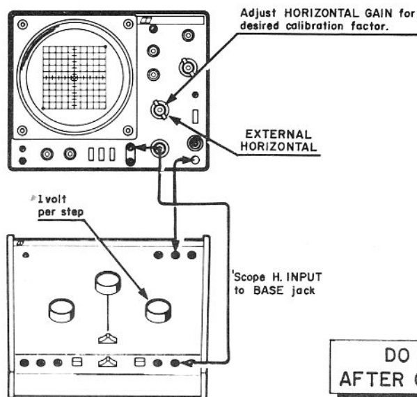
Figure 6. Oscilloscope Horizontal Calibration—Low Voltage
