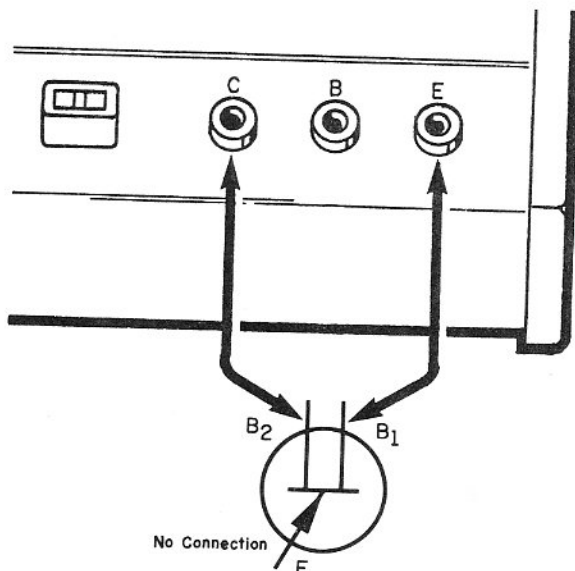
Figure 32. Measuring Interbase Resistance ( V_{BB} ) of UJT's
