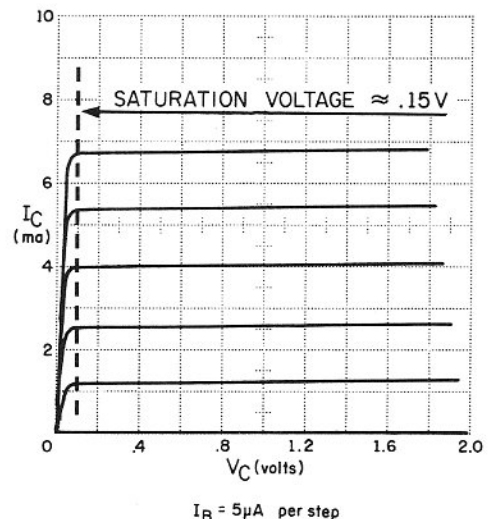
Figure 23. Saturation Voltage
