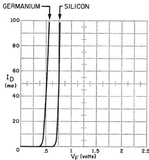
FORWARD BIAS
