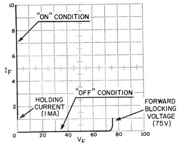
Figure 34. Testing Forward Blocking Voltage and Holding Current of SCR's
