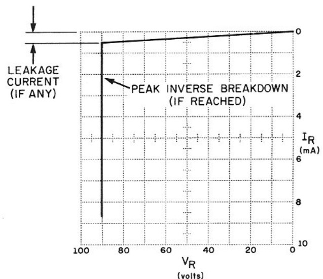
REVERSE BIAS
