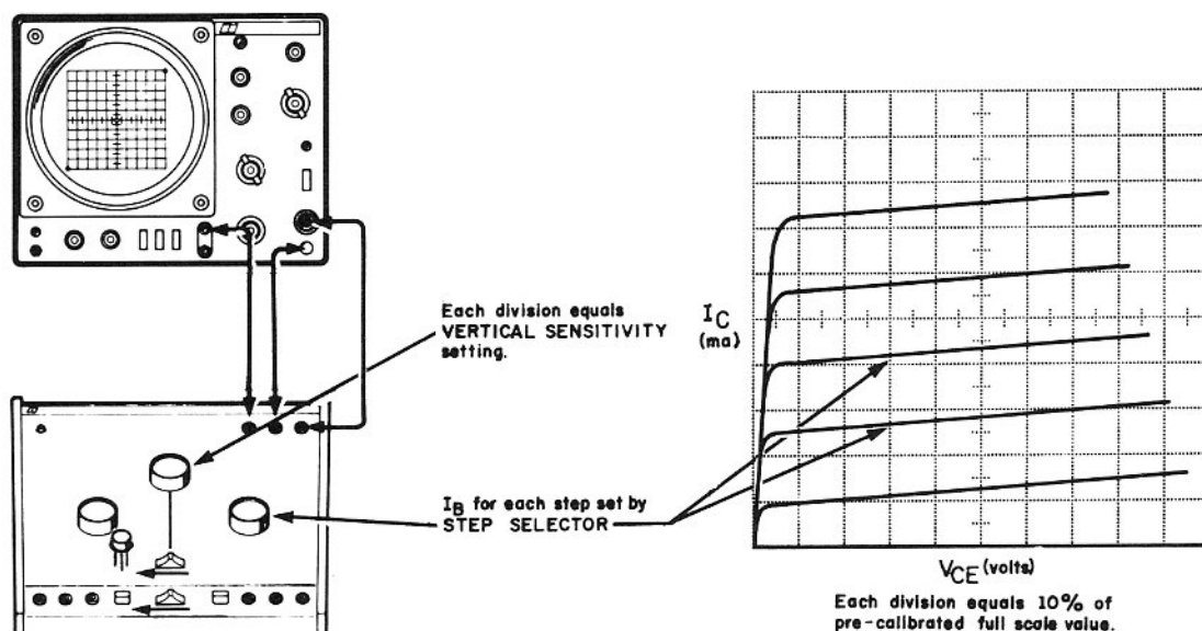
Figure 10. Typical Test of an NPN Transistor
