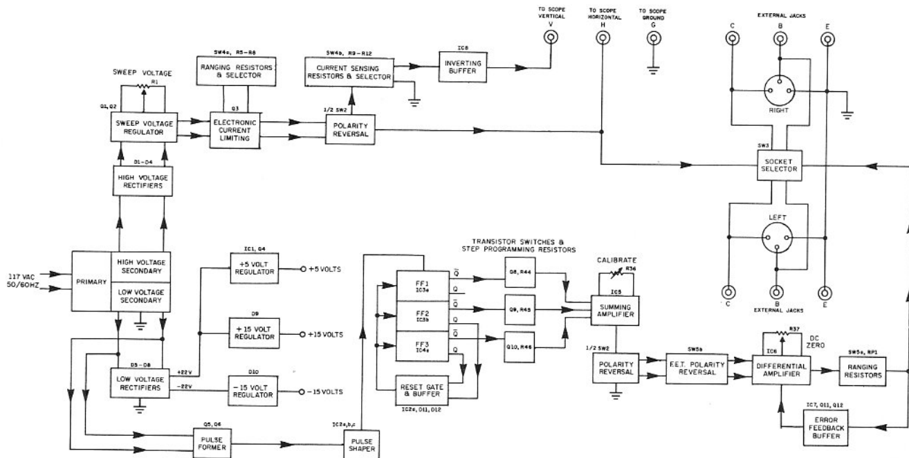
Figure 40. Block Diagram
