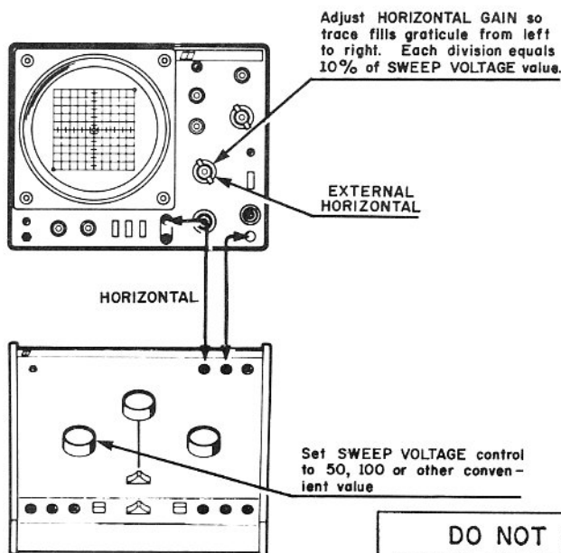
Figure 7. Oscilloscope Horizontal Calibration—High Voltage
