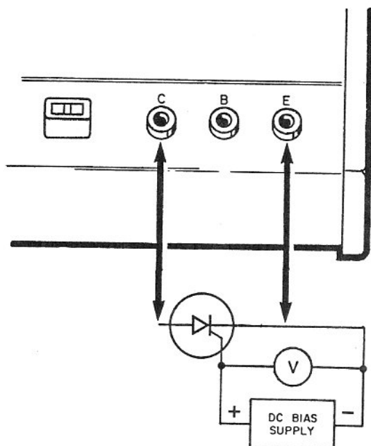
Figure 35. Testing Gate Trigger Voltage of SCR's
