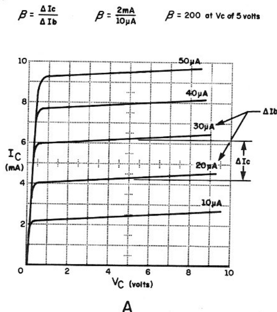
Figure 18. AC Current Gain (AC Beta) Measurement
