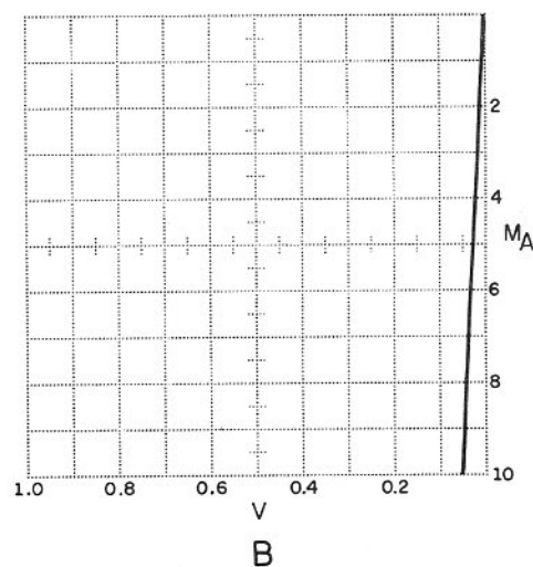
Figure 37. Tunnel Diode Characteristic Curves
