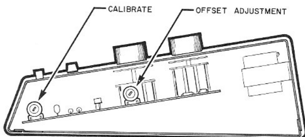
Figure 38. Location of Internal Adjustments
