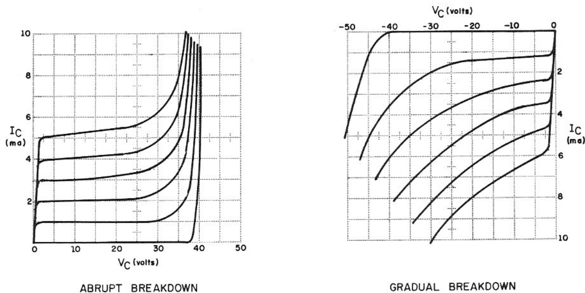
Figure 21. Typical Transistor Breakdown Curves
