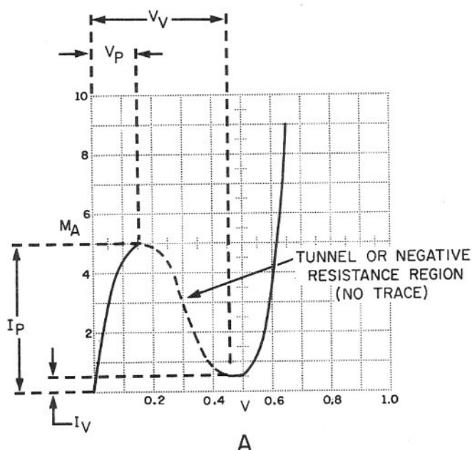
Figure 37. Tunnel Diode Characteristic Curves
