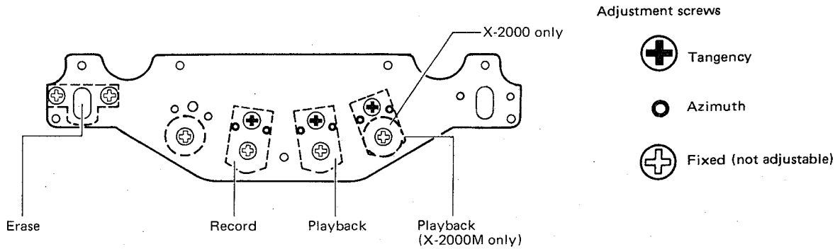
Fig. 2-21 Head arrangement
