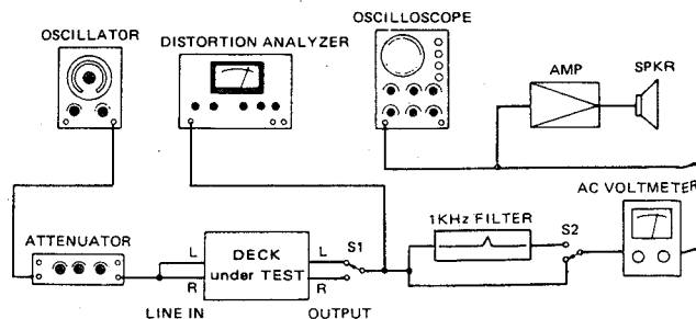
Fig. 3-3 Basic connection
