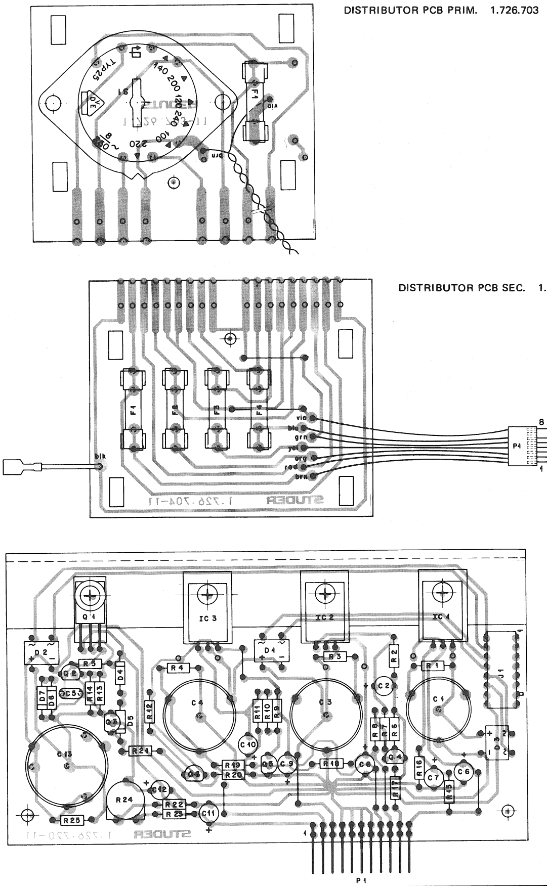
POWER SUPPLY PCB 1.726.720
