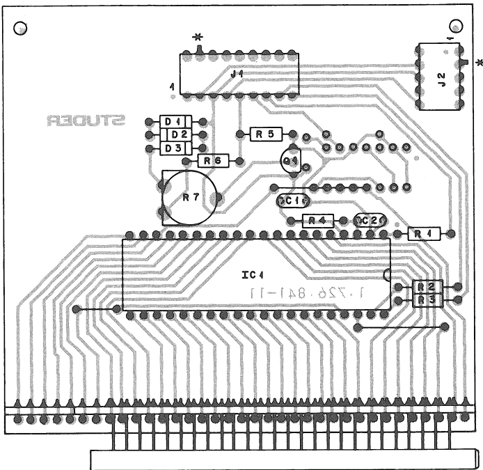
DISPLAY CONTROL PCB 1.726.841-11
