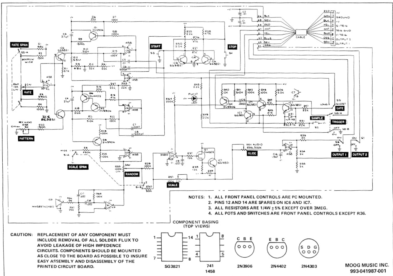
SAMPLE AND HOLD (MODEL 1125) SCHEMATIC DIAGRAM
