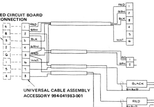
RIBBON CONTROLLER (MODEL 1150) SCHEMATIC DIAGRAM
