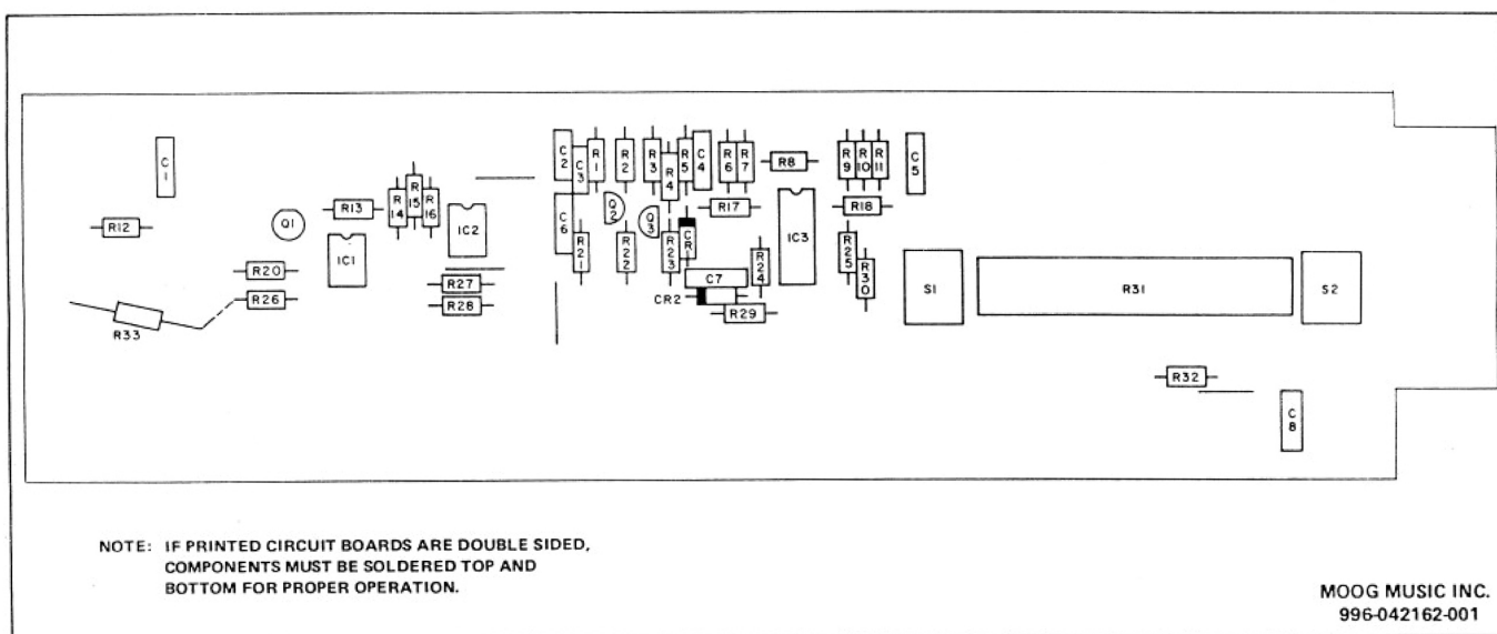
RIBBON CONTROLLER (MODEL 1150) PRINTED CIRCUIT BOARD
