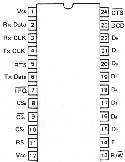
PIN CONFIGURATION
