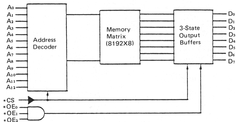
BLOCK DIAGRAM
