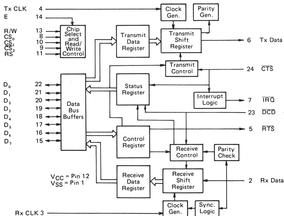
BLOCK DIAGRAM
