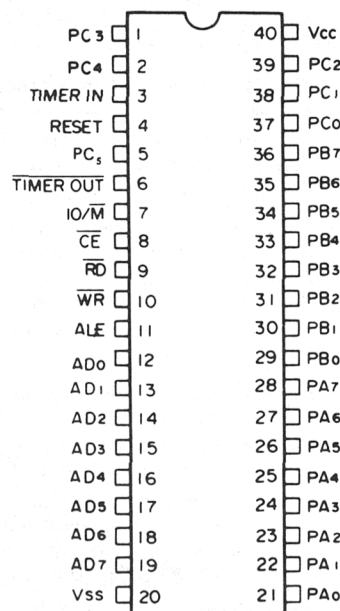
PIN CONFIGURATION
