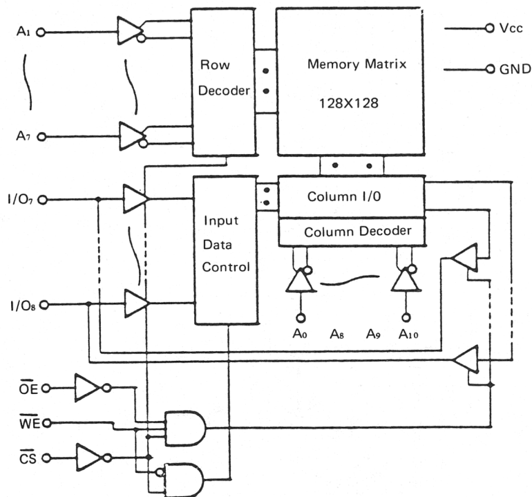
BLOCK DIAGRAM
