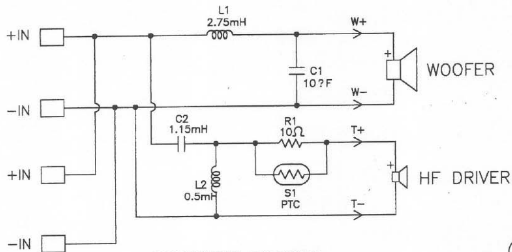
SCHEMATIC DIAGRAM CROSSOVER P/N 83707 AFTER DATE CODE 9611
