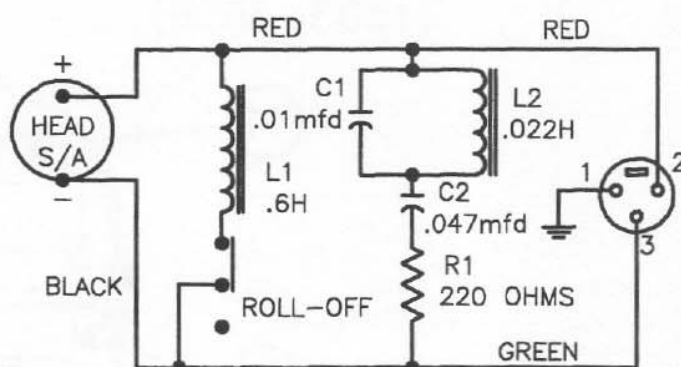
SCHEMATIC FOR N/D767
