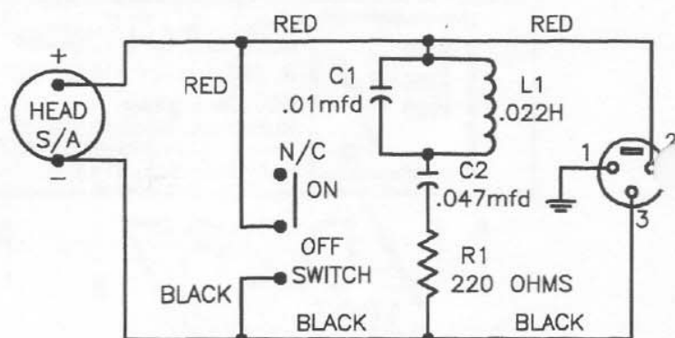
SCHEMATIC FOR N/D267S
