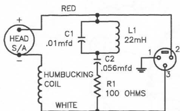
SCHEMATIC FOR N/D367
