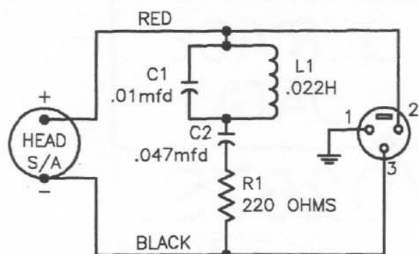
SCHEMATIC FOR N/D267
