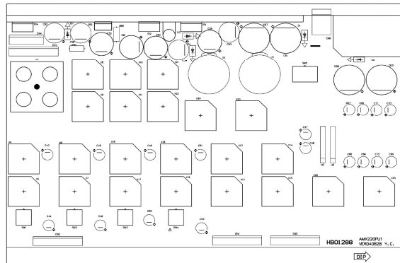
PCB: AMX220PU1 Top Overlay
