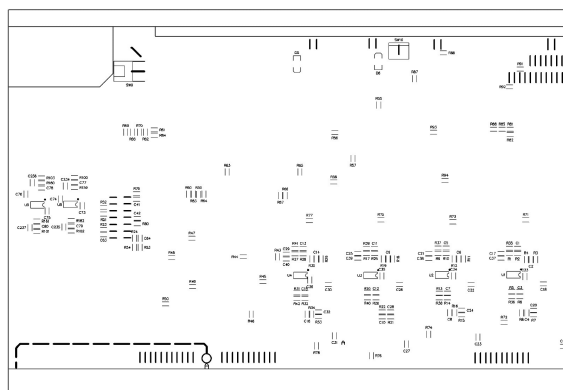
PCB: AMX220 PU1 Bottom Overlay
